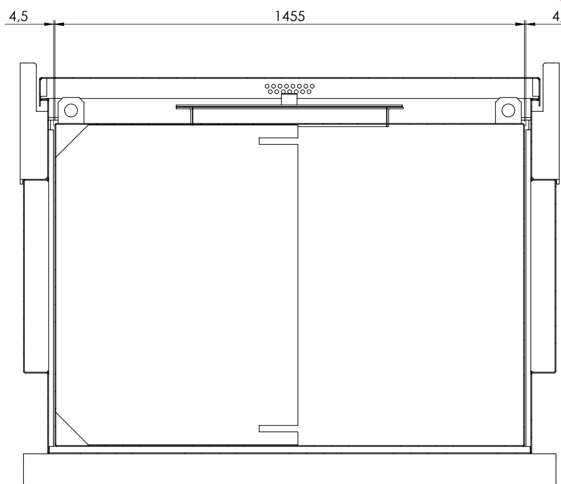
SECTION C-C
