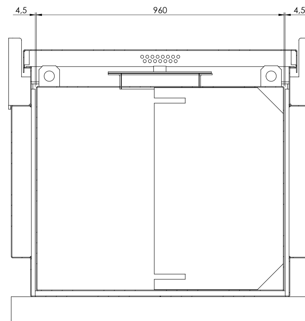
SECTION B-B
